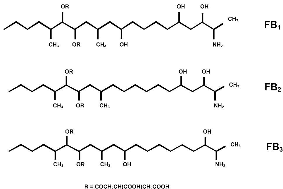
Figure 1. Structures of fumonisins B 1 , B 2 , and B 3 .
